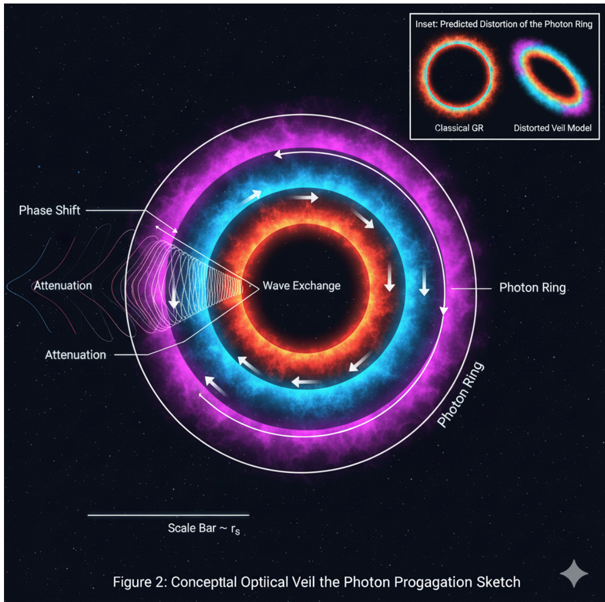
Figure 2 (placeholder). Optical veil photon propagation sketch. Example photon geodesics showing phase shift and attenuation across layers; inset: predicted distortion of photon ring.
